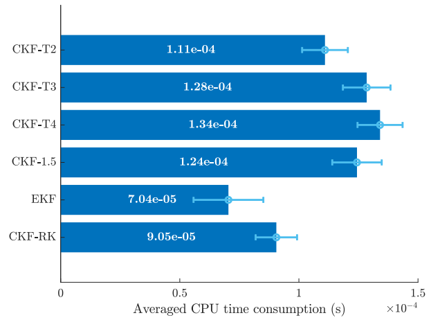
Fig. 5: Averaged CPU time from 10^6 runs on an Xeon® E3-1230v5 workstation. The error bars indicate the standard deviation of the Monte Carlo runs.
